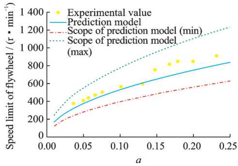
Fig.10 Relationship between a and speed limit
