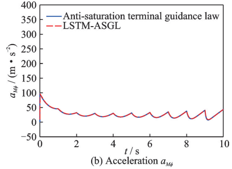
Fig.11 Acceleration comparison for a triangular maneuvering target
